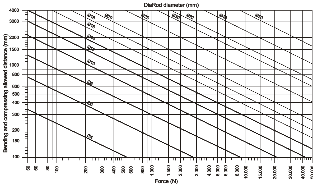
Axial load diagram
